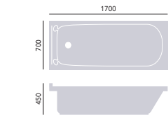
Acrylic Single Ended Fitted Bath Internal length 1514mm Internal width 567mm Height 450mm Overflow to waste 315mm Water capacity 200ltr 1700 x 700mm Solid Skin 2 taphole BRHW1770S £485
