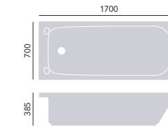
Acrylic Single Ended Fitted Bath Internal length 1510mm Internal width 574mm Height 385mm Overflow to waste 315mm Water capacity 200ltr 1700 x 700mm Solid Skin 2 taphole BDW1770S £485
