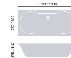
Acrylic Double Ended Fitted Bath Internal length 1540mm Internal width 559mm Height 375mm Overflow to waste 290mm Water capacity 205ltr 1700 x 750mm Solid Skin 2 taphole BDW1775D £585
