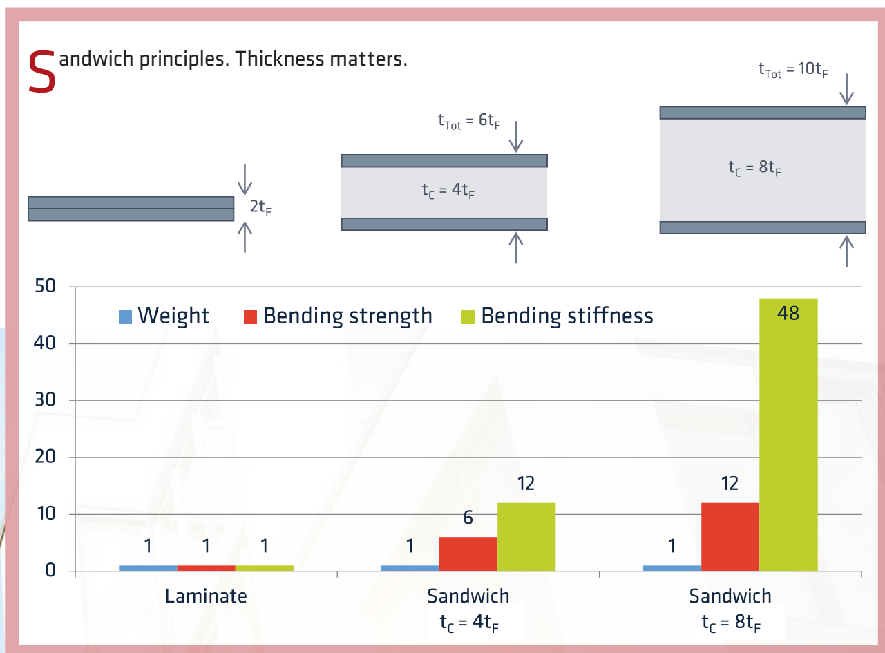
Fig. 1. Composite sandwich structures allow lightweight, strong and stiff structures that can be freely shaped in any 3D form and offer excellent insulation.
