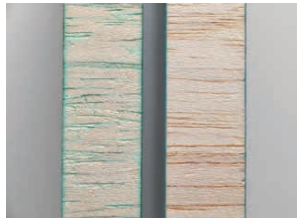
Visualization of resin uptake in cross section of infused balsa wood. Left: resin filled vessels in standard balsa. Right: BALTEK® SealX .
